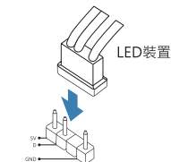
Addressable RGB LED裝置接頭 (5V_LED)
