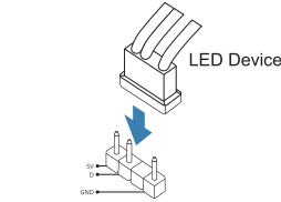
Addressable RGB LED Device Header (5V_LED)
