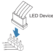
RGB LED Device Header (12V_LED)
