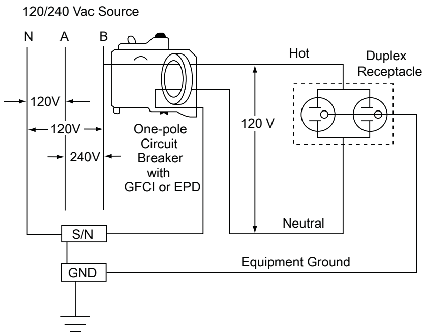
Typical One-Pole GFCI Wiring
