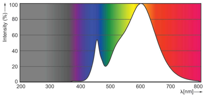
Spectral Power Distribution Colour - 7PAR20/LED/F25/830/E26/GL/DIM 120V
