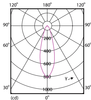
Light Distribution Diagram - 7PAR20/LED/F25/830/E26/GL/DIM 120V
