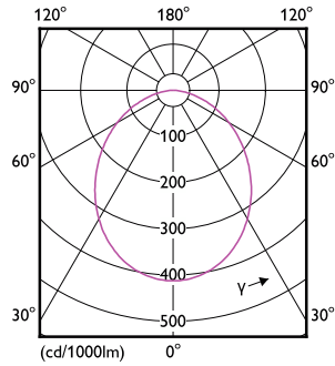
Light Distribution Diagram - DN116B LED12/3CCT 10.5W 100-277V D150 ND
