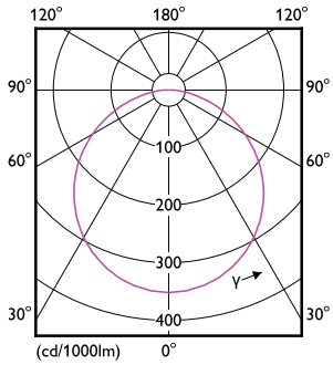
Light Distribution Diagram - DN016B LED20/NW 20W 100-240V D125 RD ND
