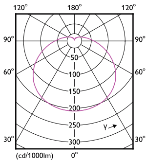
Light Distribution Diagram - LEDBulb 22W E27 6500K W A25 1PF/6 MX
