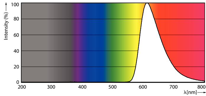
Spectral Power Distribution Colour - 8A19/LED/ORANGE/ND 120V E27 6/1FB
