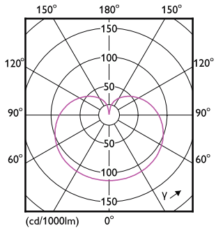
Light Distribution Diagram - 8A19/LED/ORANGE/ND 120V E27 6/1FB
