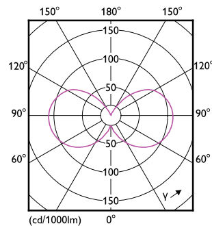
Light Distribution Diagram - LEDClassic 4.5W B11 E27 827 CL ND 1PF/10
