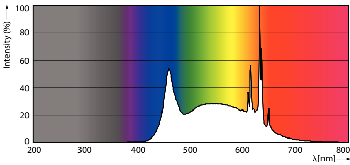
Spectral Power Distribution Colour - 8.8A19/AMB/950 DIM 120V LA
