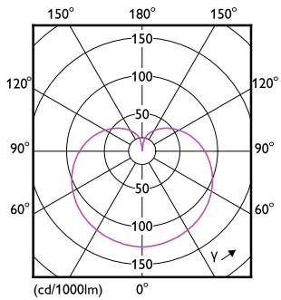
Light Distribution Diagram - 8.8A19/AMB/950 DIM 120V LA
