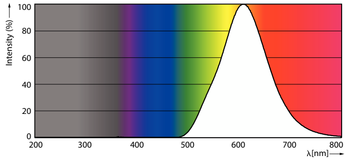
Spectral Power Distribution Colour - 8A19/LED/YELLOW/ND 120V E27 6/1FB
