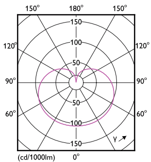
Light Distribution Diagram - 8A19/LED/YELLOW/ND 120V E27 6/1FB
