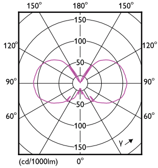
Light Distribution Diagram - 5.5F15/PER/927-922/CL/G/E26/WGX 1PF T20
