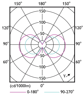
Light Distribution Diagram - LEDcapsule 40W G9 827 120V ND 1PF/6
