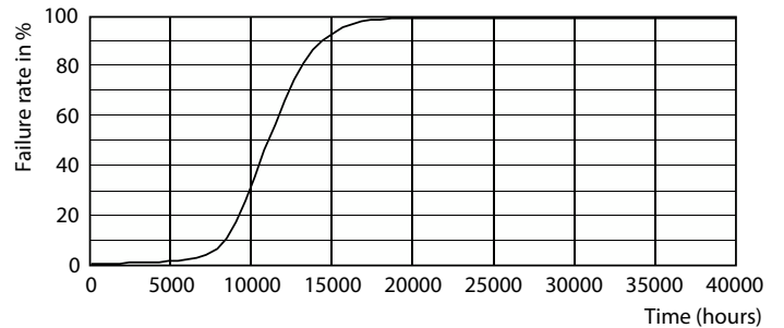
Life Expectancy Diagram - LEDcapsule 40W G9 827 120V ND 1PF/6
