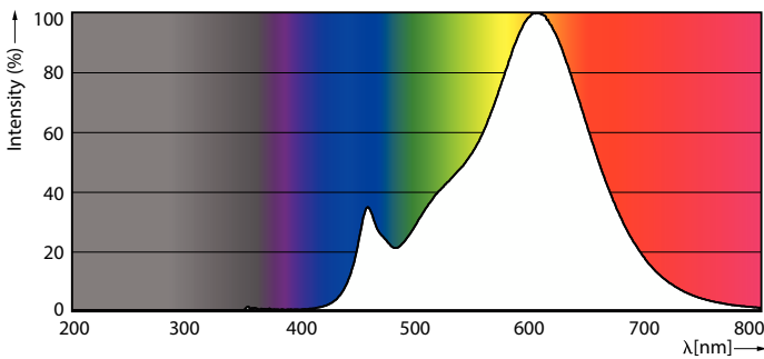
Spectral Power Distribution Colour - LEDcapsule 40W G9 827 120V ND 1PF/6
