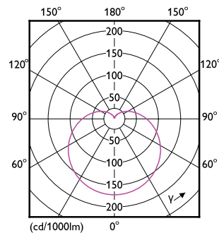
Light Distribution Diagram - LEDGlobe13-100W G30 E27 CDL W ND MX
