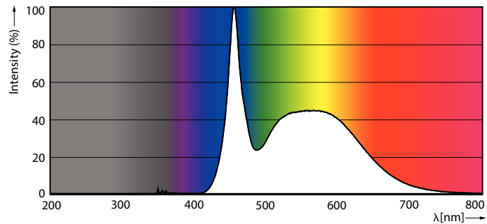
Spectral Power Distribution Colour - LEDGlobe13-100W G30 E27 CDL W ND MX
