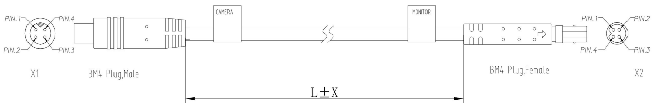
CONNECTION SCHEME:
